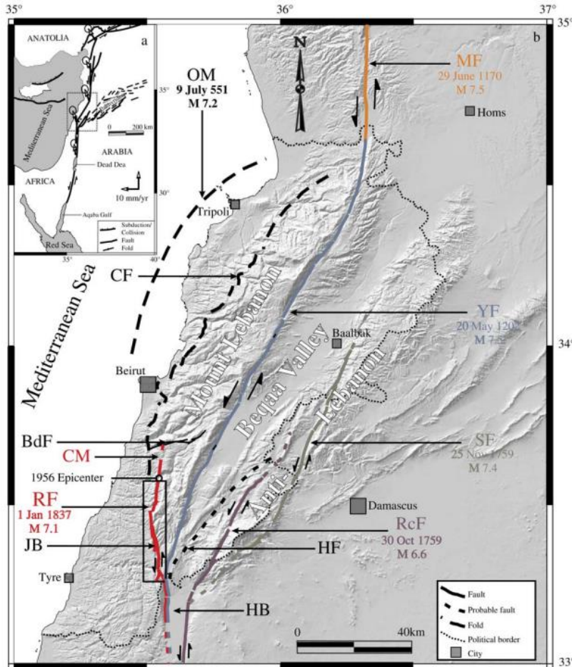
Figure 11: Lebanese Restraining Bend (Top left, Source: Nemer, T. & Meghraoui, M. (2006))
